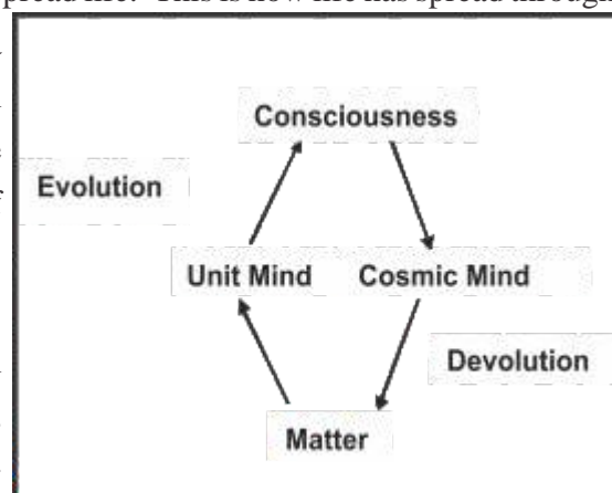
Fig.4 : Cosmic cycle of creation
