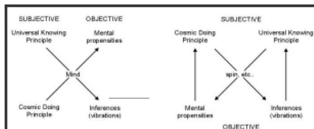
Fig. 1 - Shrii P.R. Sarkar's “Four Chambers of the Universe”, different arrangements.
