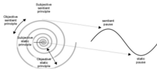
Fig. 3 - The logarithmic spiral: more than a mere analogy of the axiomatic Path into creation?
